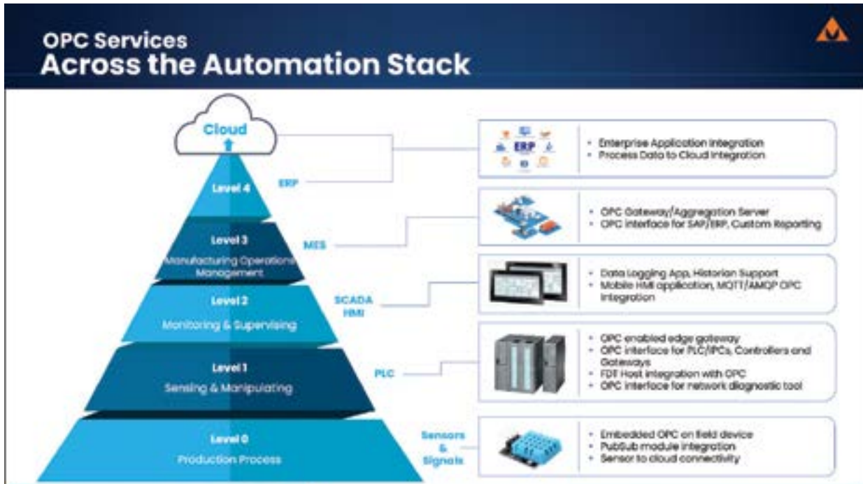
OPC UA Interoperability across the Automation Pyramid
